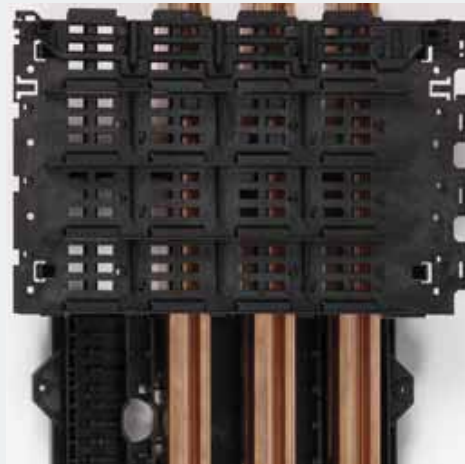
Normal withdrawable units up to 630 A and small withdrawable units up to 63A - up to 48 small withdrawable units per section for space-saving assembly
